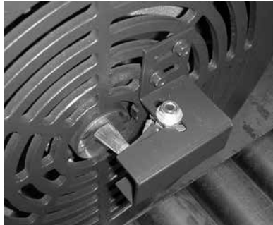
Ground Brush Opposite Drive End
